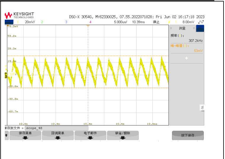
V_{ISO} ripple voltage(peak to peak): V_{INP}=5V , V_{ISO}=3.7V , I_{SO}=300mA
