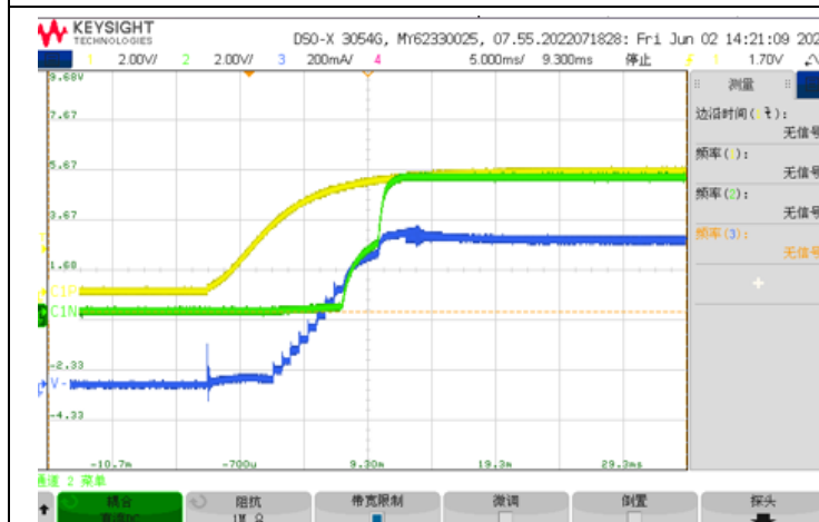
Soft-start waveform: V_{INP}=5V (yellow), V_{ISO}=5V (green), I_{ISO}=300mA (blue)
