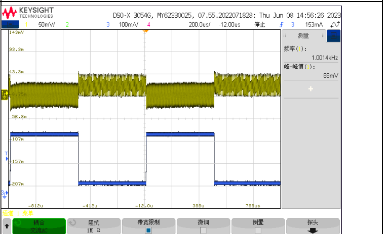
V_{ISO} ripple voltage(peak to peak): V_{INP}=5V , V_{ISO}=3.7V , I_{SO}=300mA
