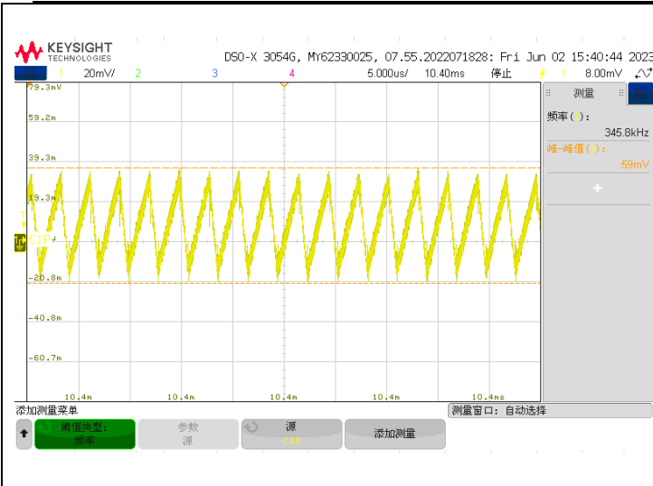
V_{ISO} ripple voltage(peak to peak): V_{INP}=5V , V_{ISO}=5.4V , I_{SO}=300mA
